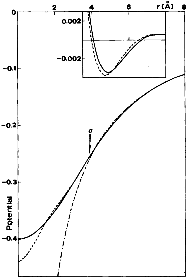
FIGURE 1 Illustrating the ORPA property (a) for the truncated potential \tilde{v}_t(r) of Ref. 1 (full curve) when compared with the potential \tilde{v}(r) of Eq. (2) (dashed curve). The arrow marks the CHS diameter \sigma for the OCP. The dot-dash curve reports for comparison the Coulomb potential -e^2/r . The inset shows on an enlarged vertical scale the total ion-ion potential in the region of its main minimum, as calculated from \tilde{v}_t(r) (full curve) and from \tilde{v}(r) (dashed curve). All potentials are in units of e^2/\text{\AA} and refer to liquid potassium at 65°C.
