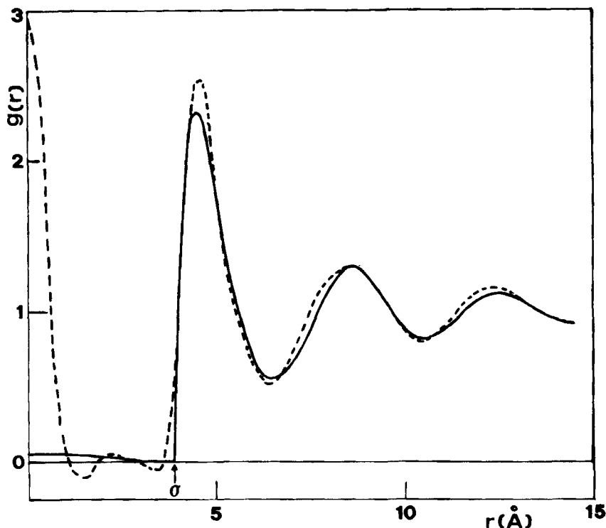
FIGURE 2 Illustrating the ORPA property (b) for the truncated potential \bar{v}_i(r) of Ref. 1. The full curve is the corresponding radial distribution function g(r) for liquid potassium at 65°C. The experimental data (dashed curve) are from M. J. Huijben and W. van der Lugt (Ref. 6): the deviations from zero at small r result from the truncation of the experimental structure factor at large k .
